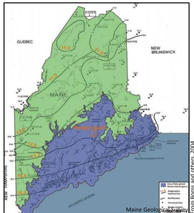
Figure 2. Deglaciation chronology for the State of Maine (in thousands of years). Location of the Bangor quadrangle and radiocarbon ages constraining timing are plotted. A reservoir correction of -600 years was applied to ages from marine samples. Areas in dark blue were isostatically depressed and flooded by sea water.
