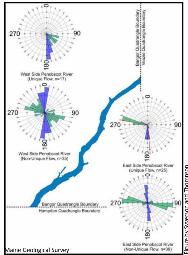
Figure 8. Rose diagrams of ice-flow indicators west and east of the Penobscot River.
