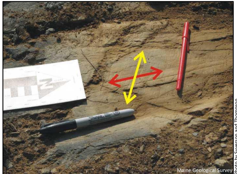
Figure 5. Striations and a groove (black marker) on phyllitic bedrock east of the Penobscot River (Interstate 395/ Parkway South interchange in Brewer, see Figure 4 for location).
