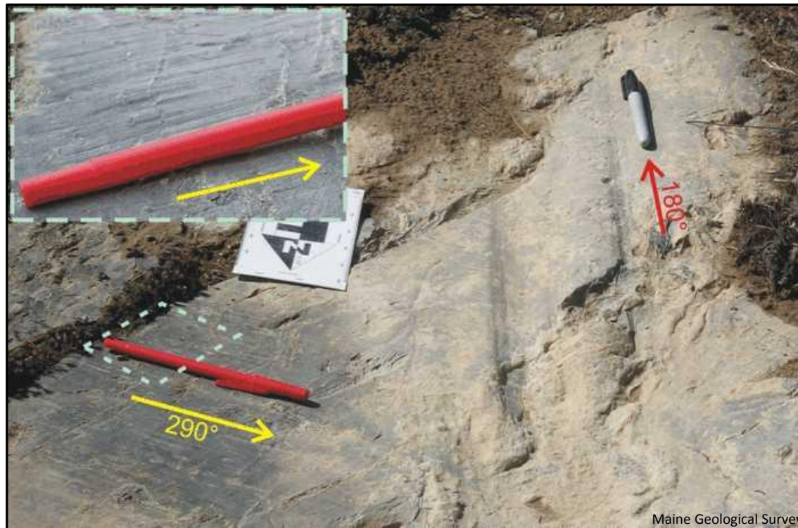
Figure 7. Large crag-and-tail features cut by smaller striations and crag-and-tail features east of the Penobscot River (Interstate 395/Parkway South interchange).
